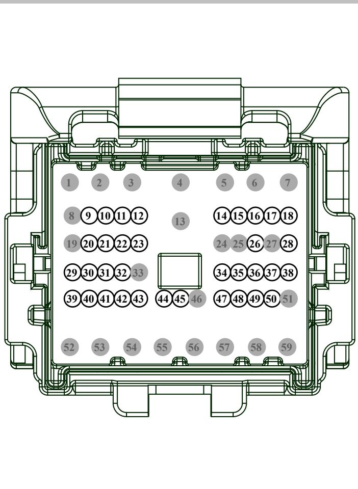
MALE Harness 14A005
