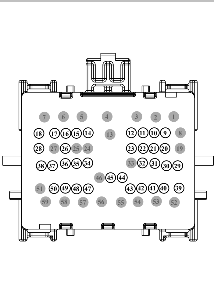
FEMALE Harness 14401
